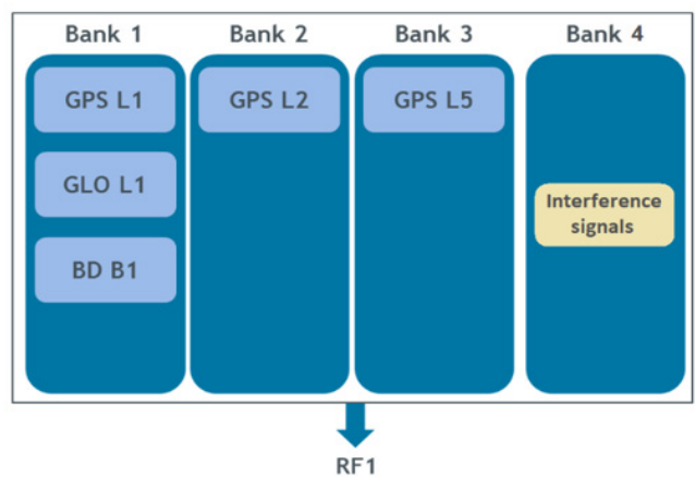
Figure 13 Triple-frequency, GNSS + interference 1RF system
